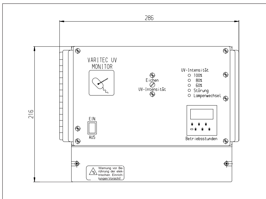
VARITEC UV-monitor
